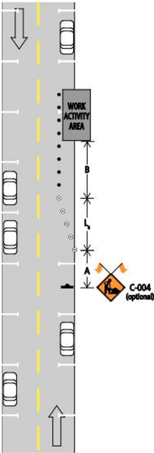
Figure 7.6: Work in Parking Lane – Urban Area
